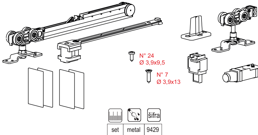
PVD TS-SELFIE 80kg FLUID mehanizam
